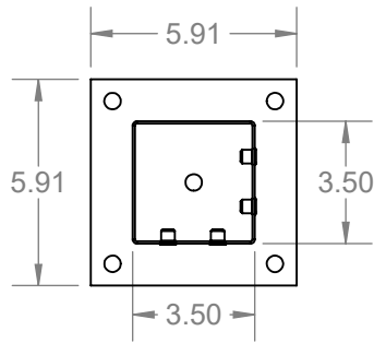
POST
