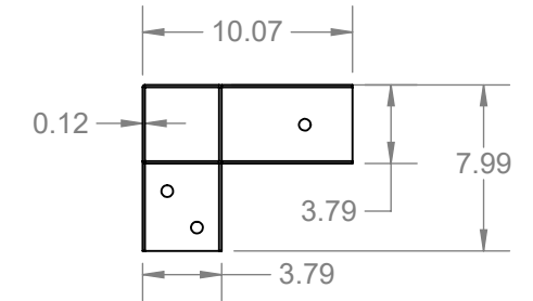
CORNER BRACE
