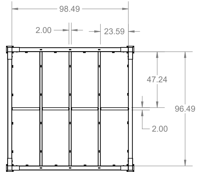
ROOF DETAILS
