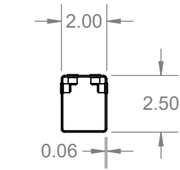
ROOF JOIST
