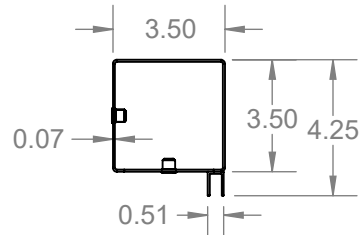
ROOF BEAM W/ JOIST CUTOUTS
